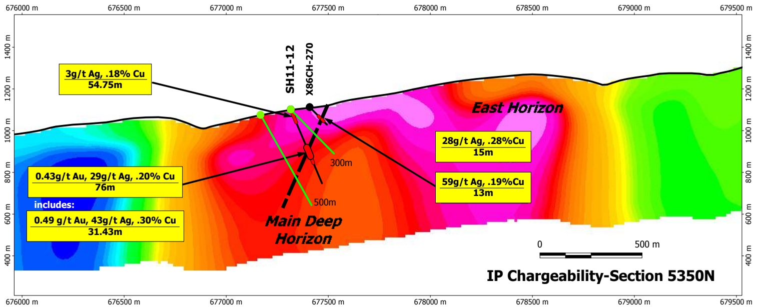
SH 11-12 cross section indicating the first two drill targets in green.
